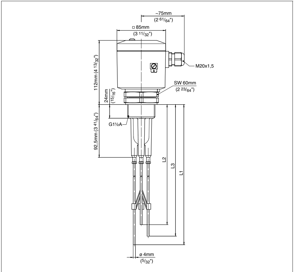
Fig. 21: VEGAKON 66 with three probes
