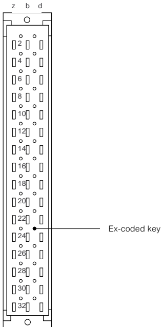
Plug-in socket, view to the plug surface
